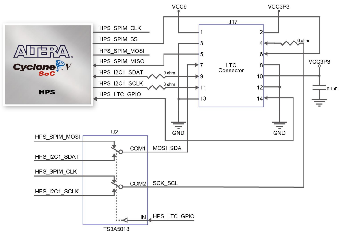
Figure 3-29 Connections between the HPS and LTC connector
