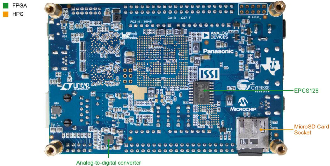
Figure 2-2 DE10-Nano development board (bottom view)
