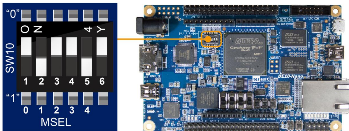
Figure 3-1 DIP switch (SW10) setting of Active Serial (AS) mode.
