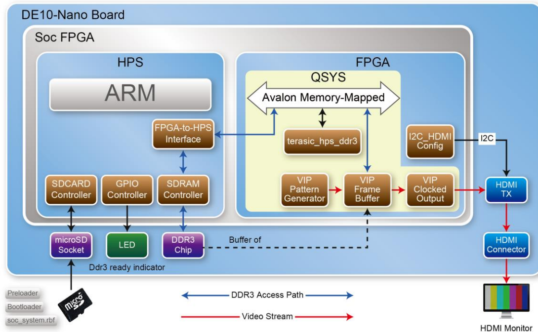
Figure 5-9 Block Diagram of the DDR3_VIP Demonstration
