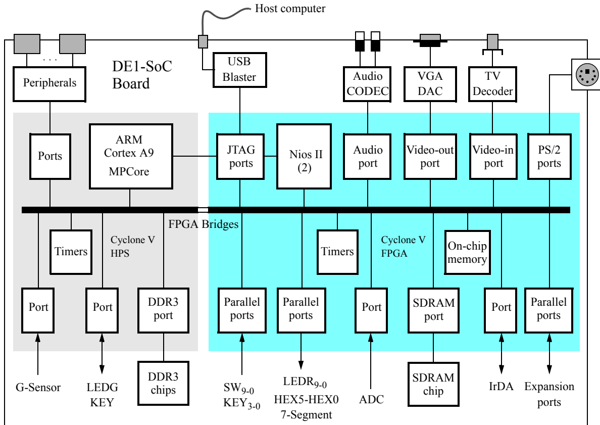
Figure 1. Block diagram of the DE1-SoC Computer.
